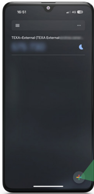
Figure 2 - Google Authenticator
